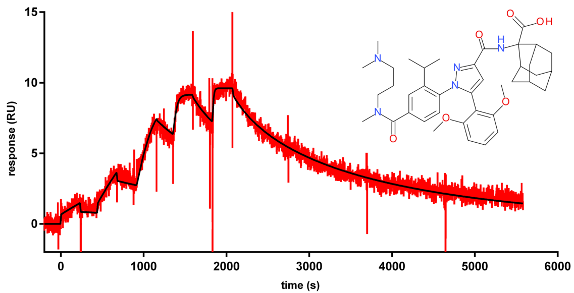
S1 Fig. Titration of SR142948 antagonist up to 25 nM over the NTS1-H4 surface monitored in single cycle kinetic mode (red curve) overlaid with the calculated curve for a one-to-one interaction (black curve) and structure of the SR142948 antagonist.
