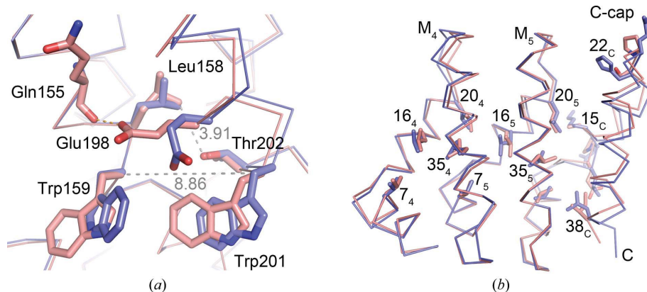
Figure 4 Superposition of Y_{III}M_5A_{III} (third-generation C-cap; PDB entry 4plq; salmon) on Y_{III}M_5A_{II} (second-generation C-cap; blue). ( a ) Residues at the M_3 – M_4 interface. General distances and hydrogen bonds are shown as grey and orange dotted lines, respectively. Distance values refer to Y_{III}M_5A_{III} . The superposition is based on all C \alpha atoms from M_3 . ( b ) Residues at the M_5 –C-cap interface. Numbers refer to positions in the repeat (Fig. 1c), with subscripts indicating the internal repeat number or the C-cap. Side chains of all residues that differ between Y_{II} and Y_{III} and some residues from the hydrophobic core are shown in stick representation. The superposition is based on all C \alpha atoms from M_5 .
