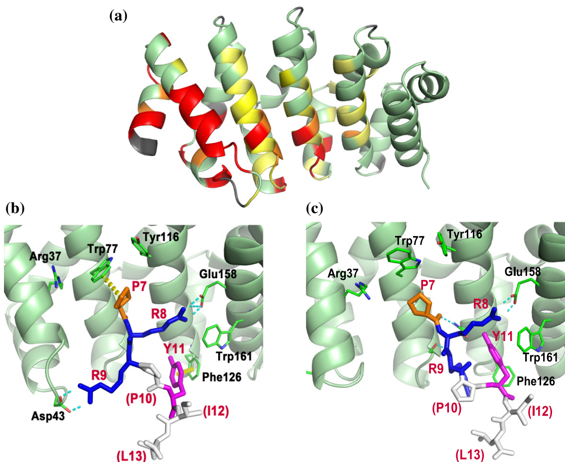
Fig. 4. Interaction of NT with the minimal binder Y_I MR^1 R^2 A_{II} . (a) Backbone amide CSPs induced by addition of 2 eq. NT are highlighted: red, resonances that could only be assigned in the presence of NT; orange, CSPs \Delta\delta_{HN} > \Delta\delta_{HN} + \sigma ; yellow gradient, \Delta\delta_{HN} > \Delta\delta_{HN} ; gray, Pro and unassigned residues. (b) and (c) display the two most populated binding poses obtained from MD simulations with the parallel AutoDock orientation as starting point. The lowest-energy ligand structure is depicted as sticks with non-interacting residues Pro10 NT , Ile12 NT , and Leu13 NT in gray and interacting residues in orange, blue, and magenta.
