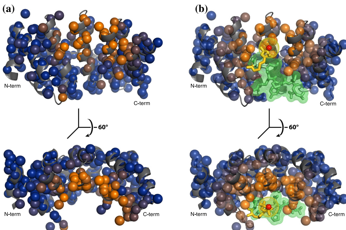
Fig. 5. Interaction of Y_1MR^1R^2A_{11} with NT-K6C as probed by PREs. The protein backbone is in ribbon representation (gray), individually tracked atoms are shown as spheres, and peptide bonds are depicted as sticks. Color intensity of the spheres is proportional to (real or simulated) PRE effect in blue-to-orange gradient. (a) Experimental PRE effect (orange, >80% loss of signal). (b) NTK6C-13 poses as predicted by AutoDock Vina. Color intensity on the receptor correlates with distance to the nitroxide radical (orange, <10 Å; blue, >22 Å). The docked peptide is delineated (green sticks and van der Waals surface; hydrogens are hidden for clarity) with the coupled MTSL spin label (yellow sticks). The nitroxide moiety (red sphere) is the source of the PRE effect as symbolized by yellow dots.
