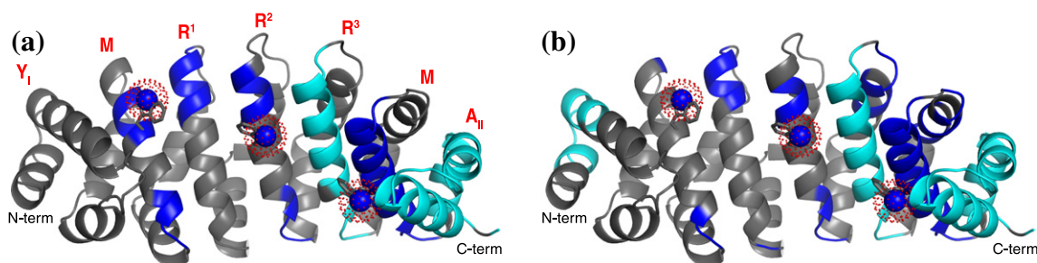
Fig. 2. Assignments of Y I MR 1 R 2 R 3 MA II in the absence (a) and presence (b) of NT. Prolines and unassigned residues are colored gray; assigned Trp indole amide moieties, used to locate repeats involved in binding NT by CSP (see Fig. 3b), are shown as spheres inside a red-dotted cloud. A Y I MR 1 R 2 R 3 MA II assignment based on conventional strategy (cyan) and additional assignments achieved by fragment strategy (blue); modules are schematically labeled for reference (red). (b) Y I MR 1 R 2 R 3 MA II assignment in the presence of 2 equivalents of NT, using the conventional (cyan) or fragment strategy (blue).
