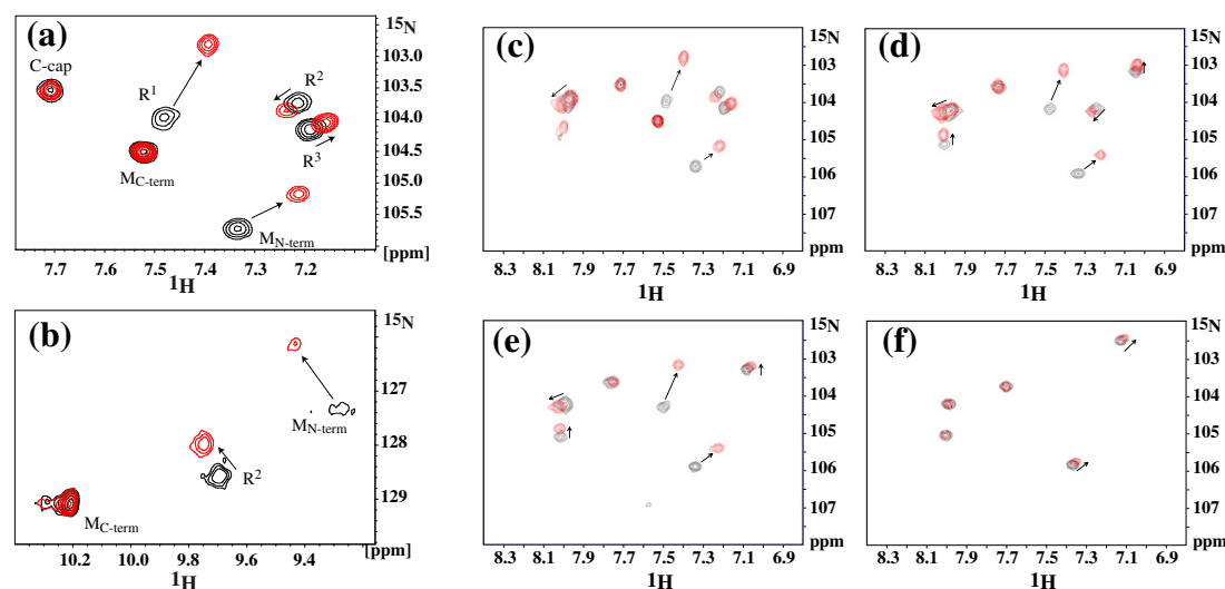
Fig. 3. CSPs induced by NT in Y_1MR^1R^2R^3MA_{II} (a–c) and its truncated versions (d–f): CSP in [^{15}N, ^1H] -HSQC spectra displaying the Gly (a) and indole Trp (b) regions of Y_1MR^1R^2R^3MA_{II} in the absence (black) and presence of two equivalents of NT (red). Similarly, expansions of the Gly region in [^{15}N, ^1H] -HSQC spectra of full-length Y_1MR^1R^2R^3MA_{II} (c), Y_1MR^1R^2R^3A_{II} (d), Y_1MR^1R^2A_{II} (e), and Y_1MR^1A_{II} (f) are depicted with and without NT. For full spectra see Figs. S4 and S5.
