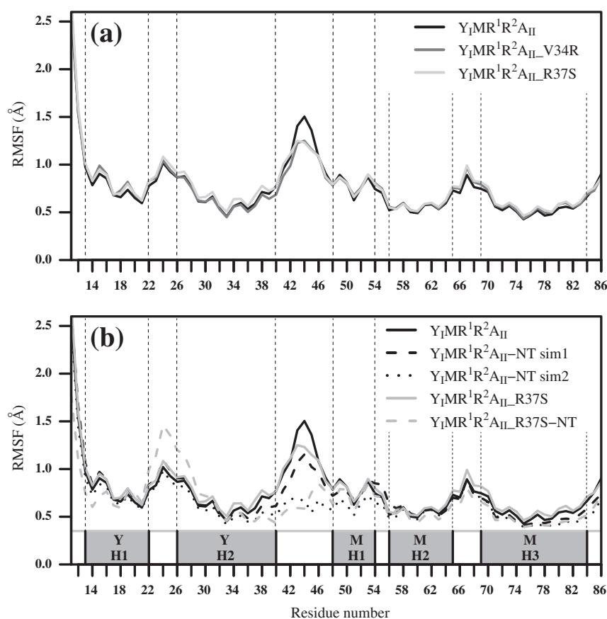
Fig. 8. Flexibility of N-cap and first internal repeat. (a) Profiles of RMSF of C \alpha atoms of selected Y 1 MR 1 R 2 A II variants. (b) Profiles of RMSF of C \alpha atoms of Y 1 MR 1 R 2 A II and Y 1 MR 1 R 2 A II _R37S in the presence and absence of NT. All RMSF are calculated on 2-ns segments during the second half of each simulation (i.e., between 1 \mu s and 2 \mu s), and then averaged. The location of helices is indicated by gray bars.
