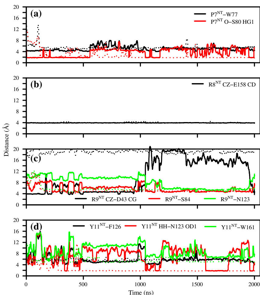
Fig. 6. Intermolecular contacts. Time evolution of distances among Pro7 NT , Arg8 NT , Arg9 NT , and Tyr11 NT and main interacting residues of Y I MR 1 R 2 A II , when NT(7-13) is in the parallel orientation. Continuous and dotted lines represent two independent runs. In (a) and (d), Pro7 NT -Trp77, Tyr11 NT -Phe126, and Tyr11 NT -Trp161 distances are calculated between the center of masses of the aromatic or pyrrolidine rings. In (c), Arg9 NT -Ser84 and Arg9 NT -Asn123 distances are calculated between the centers of masses of the two residues.
