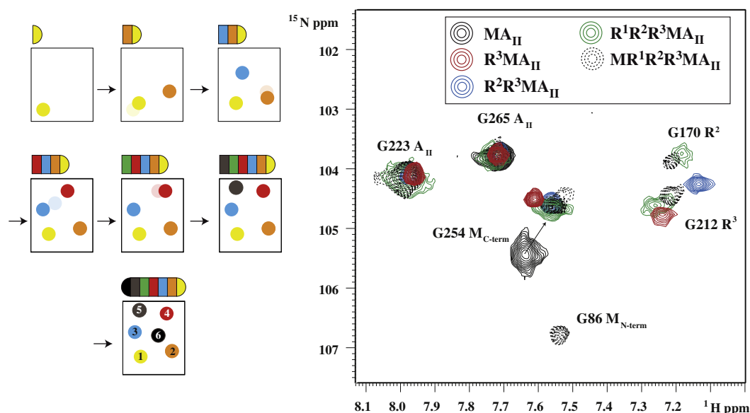
Fig. 1. Assignment strategy for fragments of increasing size. The expansion depicts an overlay of the region of signals of Gly residues. For example, the signal of Gly254, part of the MA II fragment, slightly moves toward a different position in longer fragments. In the scheme on the left, the location of the peak in the smaller fragment is shown with less opacity to indicate the peak positions in the previous protein with one repeat less. On the other hand, the signal of Gly86 only appears in the spectrum of the longest fragment MR 1 R 2 R 3 MA II .
