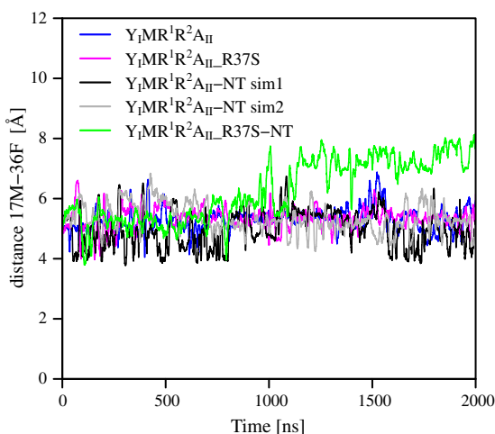
Fig. 9. Temporal evolution of the distance between the S^\delta atom of Met17 and the center of the phenyl ring of Phe36.
