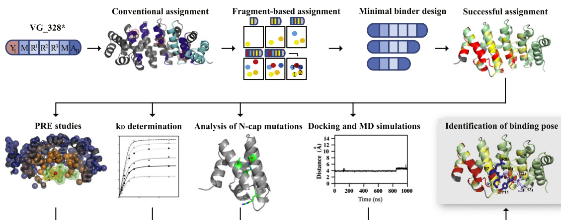
Fig. 10. Workflow of the multidisciplinary approach to the elucidation of the binding mode of the NT(7-13) peptide with the designed ArmRP Y I MR 1 R 2 A II .
