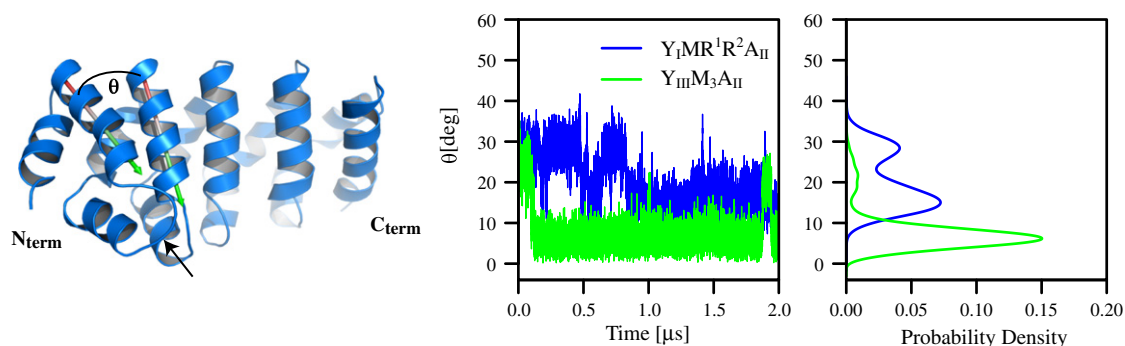
Fig. 7. Inter-helical angle between helix 2 of the N-cap and helix 3 of the first internal repeat. (Left) The angle \theta reflects the orientation of the N-cap relative to the first internal repeat. The black arrow indicates the position of G44 in the loop. (Middle and right) Time series and probability density, respectively, of the inter-helical angle \theta for Y_I MR^1 R^2 A_{II} (blue lines) and Y_{III} M_3 A_{II} (green lines).
