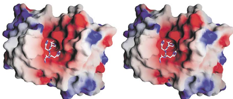
Figure 9. The peptide binds in a deep pocket with a strong negative surface potential of the antigen-binding site calculated and displayed with GRASP. 31 Negative potential is colored in red; positive potential is colored in blue. The peptide is colored by atom type C (white), N (blue), O (red).
